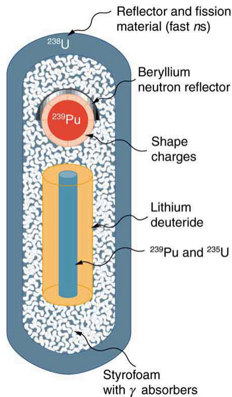
Figure 32.31 This schematic of a fusion bomb (H-bomb) gives some idea of how the ^{239}\text{Pu} fission trigger is used to ignite fusion fuel. Neutrons and \gamma rays transmit energy to the fusion fuel, create tritium from deuterium, and heat and compress the fusion fuel. The outer shell of ^{238}\text{U} serves to reflect some neutrons back into the fuel, causing more fusion, and it boosts the energy output by fissioning itself when neutron energies become high enough.
